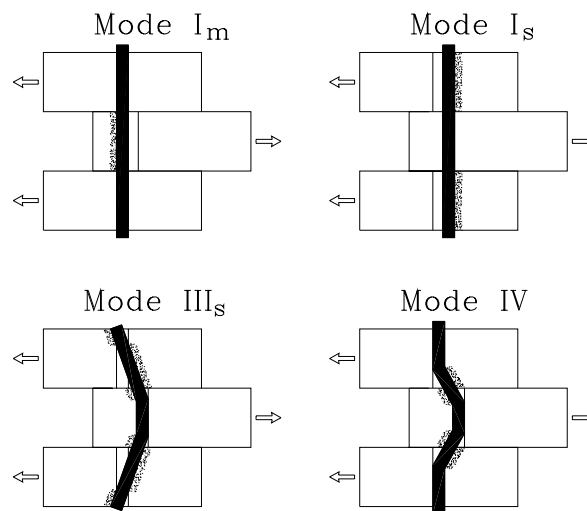
Figure 1-2 - NDS Double Shear Failure Modes
