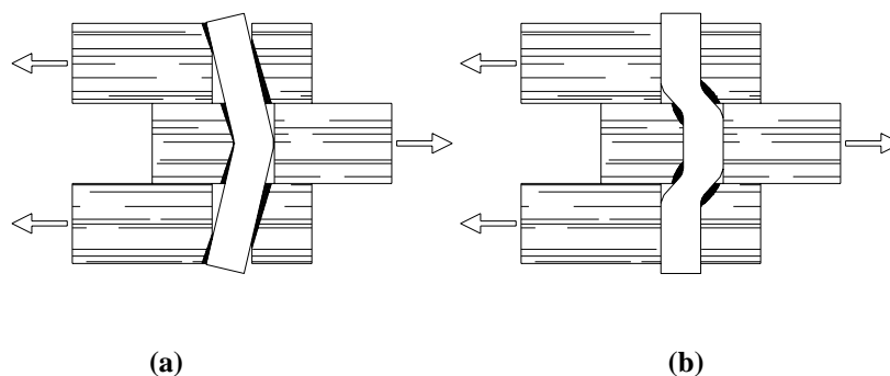
Figure 2-5 - (a) Peg Bending and (b) Shear Failures
